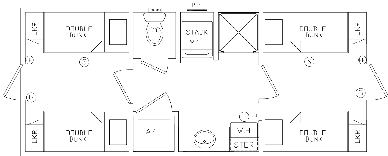
11'x26' 8 MAN SLEEPER
